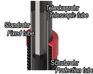
⑥ Rohre Tubes
